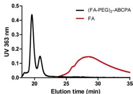
Figure 3. GPC chromatograms (UV signal at 363 nm) of (FA-PEG) 2 -ABCPA and free folic acid (FA).
