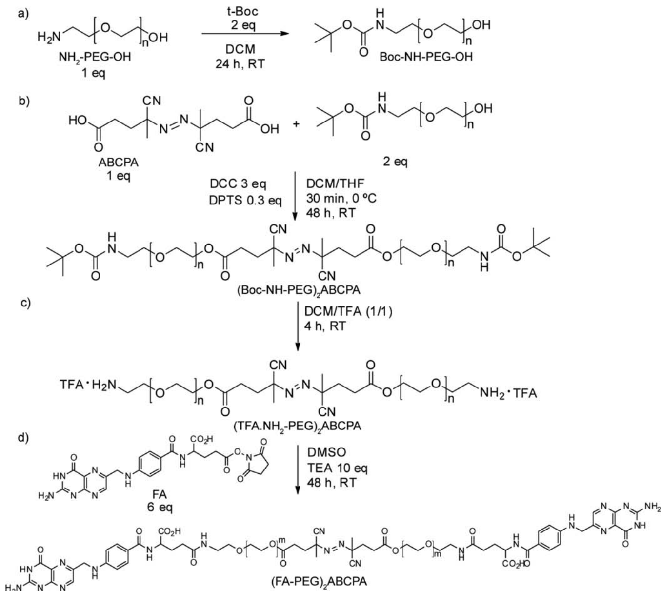
Scheme 1. Synthesis Route of (FA-PEG) 2 -ABCPA
