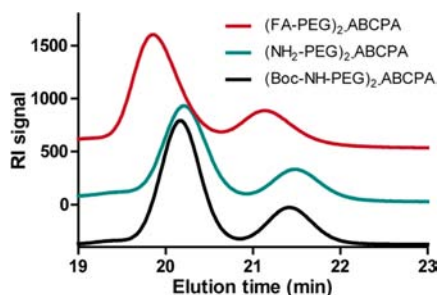
Figure 1. GPC chromatograms (RI signal) of (Boc-NH-PEG) 2 -ABCPA, (NH 2 -PEG) 2 -ABCPA, and (FA-PEG) 2 -ABCPA.
