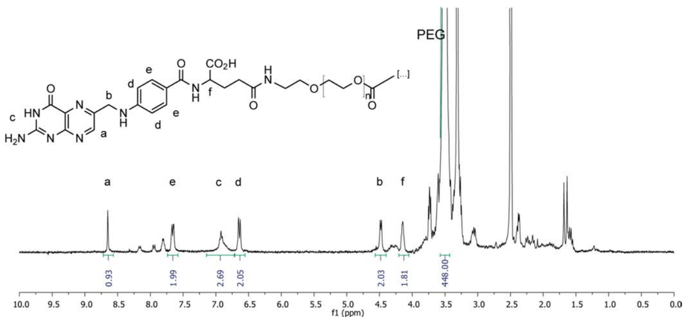
Figure 2. 1 H NMR spectrum of (FA-PEG) 2 -ABCPA in DMSO.
