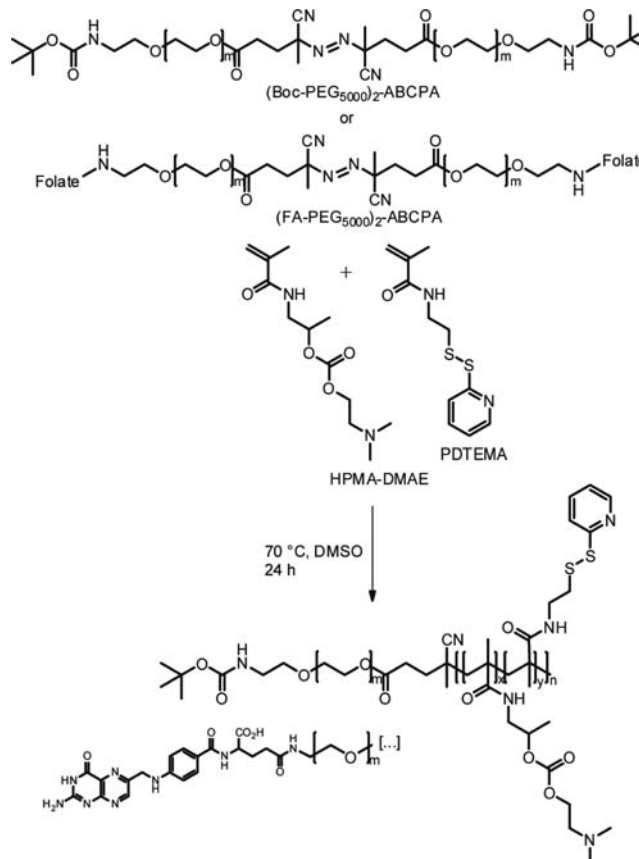
Scheme 3. Synthesis of pHDP-PEG-FA and pHDP-PEG
