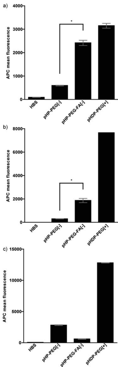
Figure 5. Mean fluorescence intensity per cell after different Cy5-pDNA polyplexes were incubated with HeLa cells (FR +) (a), OVCAR-3 cells (FR +) (b), and A549 (FR -) (c) for 2 h at 37 °C (pDNA dose was 10 \mu\text{g}/\text{mL} , 10%wt Cy5 pDNA). Results are expressed as mean \pm SD ( n = 3 ). * p < 0.01 ( t test).
