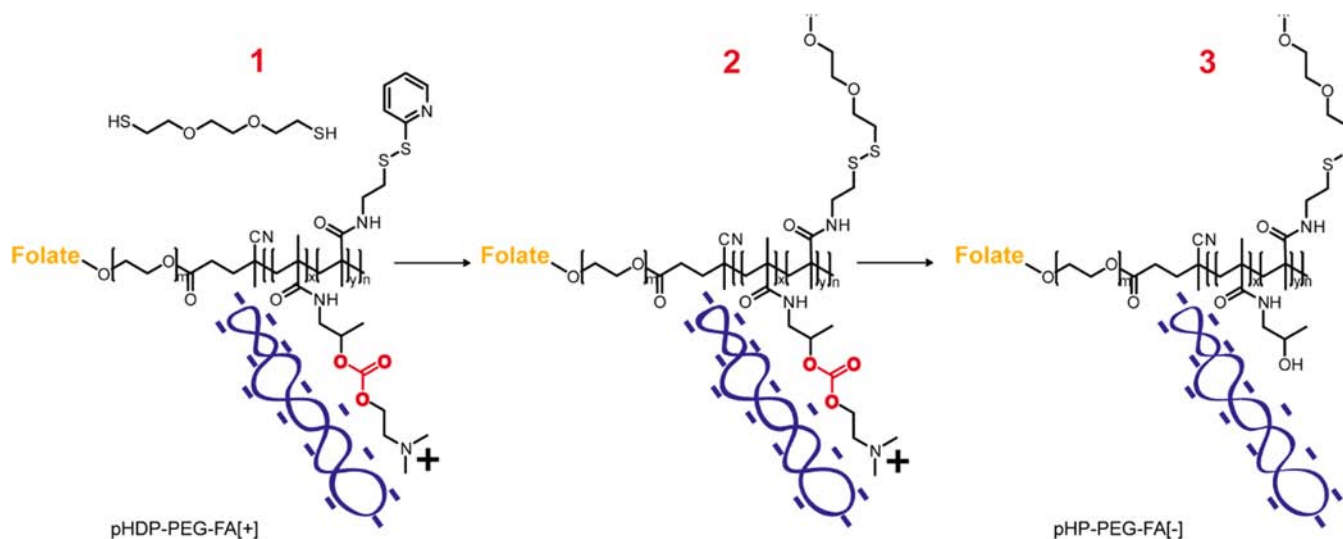
Scheme 3. Synthesis of pHDP-PEG-FA and pHDP-PEG
